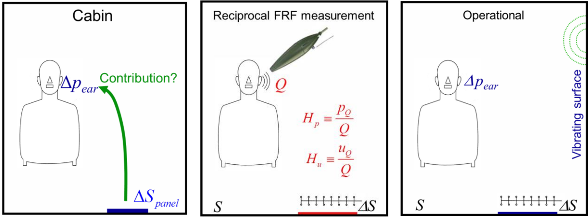
Figure 7a – Panel contribution analysis, PCA
