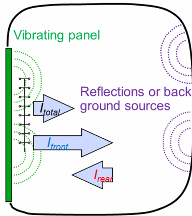
Figure 6a – Net intensity is a summation of positive and negative going intensities
