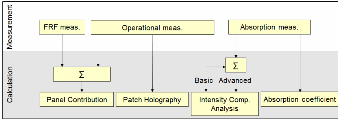
Figure 10 – Overview of the various measurement combinations for the four hand held array applications
