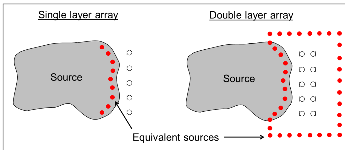
Figure 1a – ESM modeling using Single Layer Array, Figure 1b – ESM modeling using Double Layer Array
