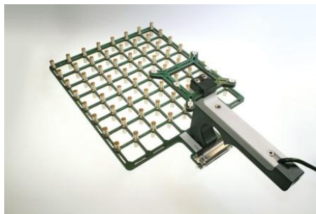
Figure 3a – Double layer array with 8x8x2 microphones
