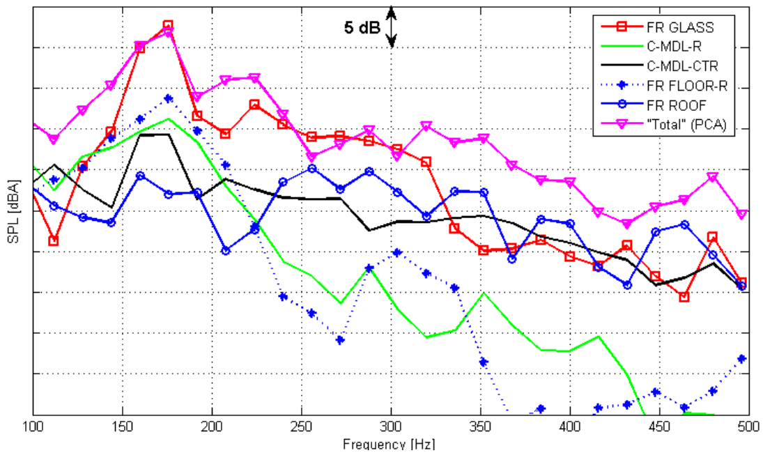
Figure 9 – Panel contribution analysis at driver's position inside a passenger vehicle. Below 325Hz the wind shield (red curve) is the dominating contributor. Above 325 Hz the front roof (blue curve) becomes a significant contributor at several frequencies
