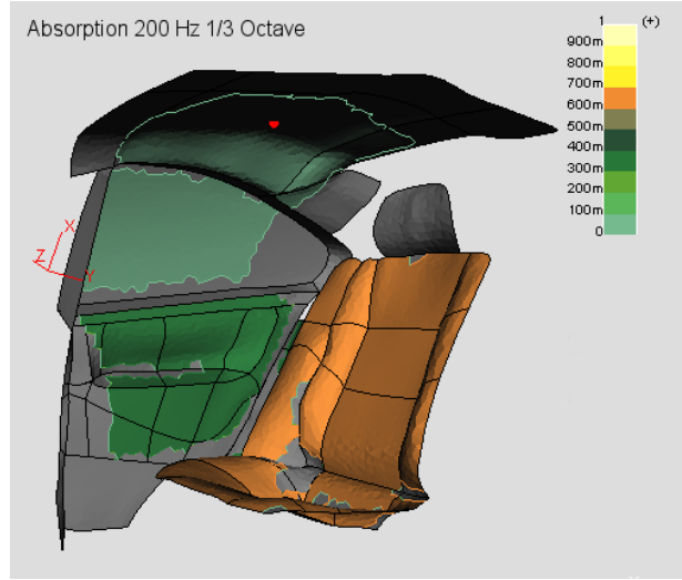
Figure 5 – A contour plot of the estimated absorption coefficient of seat, door, window and roof in a car cabin. Results shown for the 200 Hz 1/3-octave band are averaged over the respective areas.
