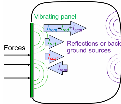
Figure 6b – Positive intensity is a summation of radiated and scattered intensities
