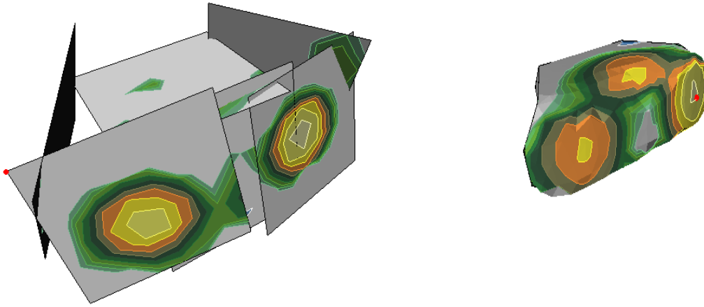
Figure 4a – Six measurement patches, Figure 4b – Patch Holography / Conformal Mapping results
