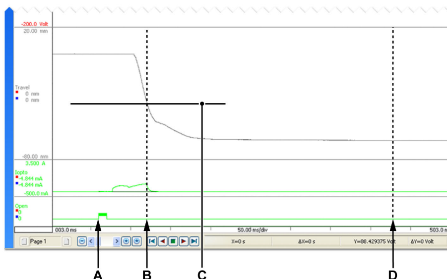
Figure 3.10: Display - Location of contact separation/touch
