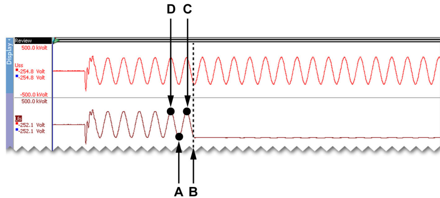
Figure 6.10: Display - Calculation on the voltage before contact separation (RMS Crests)
