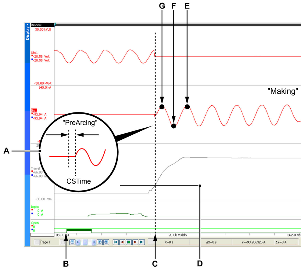
Figure 5.10: Display - Making current calculation
