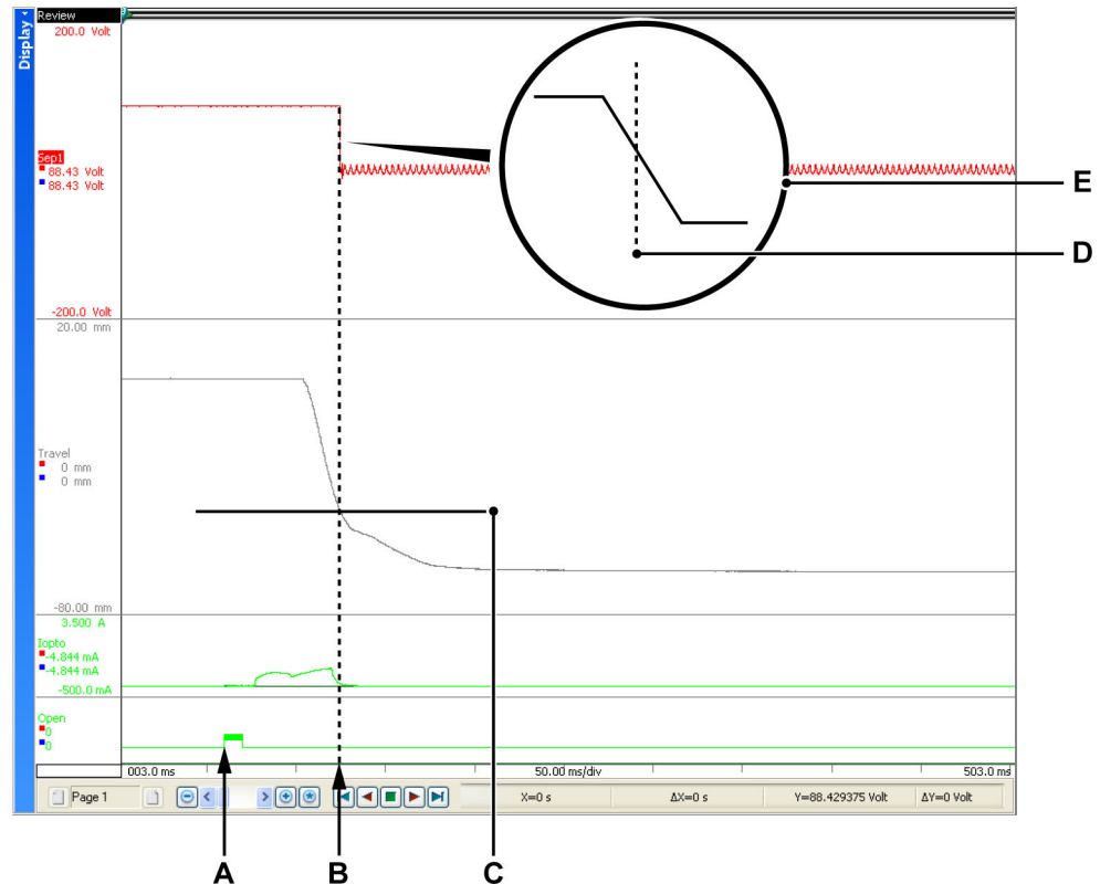
Figure 4.6: Display - Open event - Calculations on No-Load
