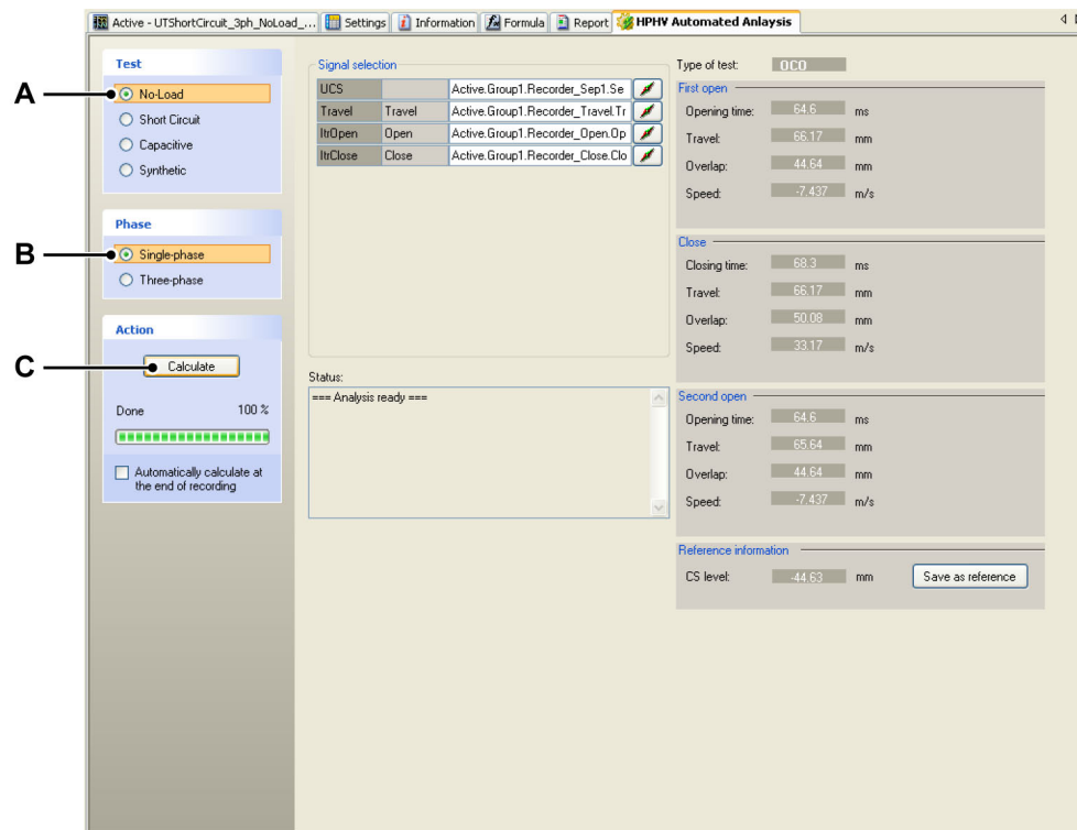
Figure 4.2: HPHV Automated Analysis Sheet - Initial calculation process - No-Load
