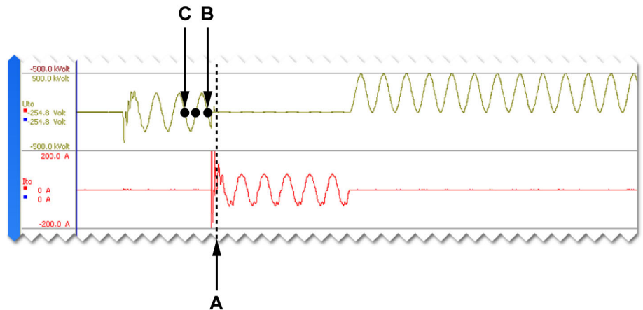
Figure 6.19: Display - RMS Time
