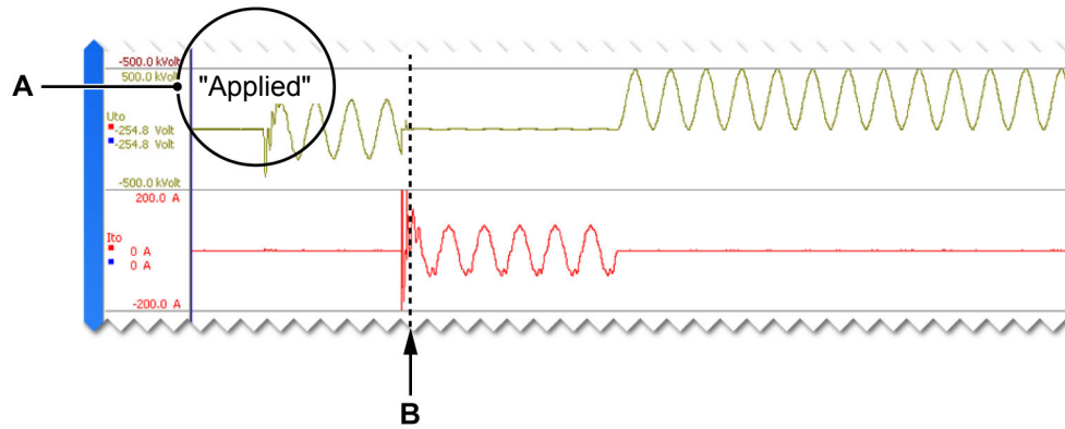
Figure 6.18: Display of an applied voltage calculation process
