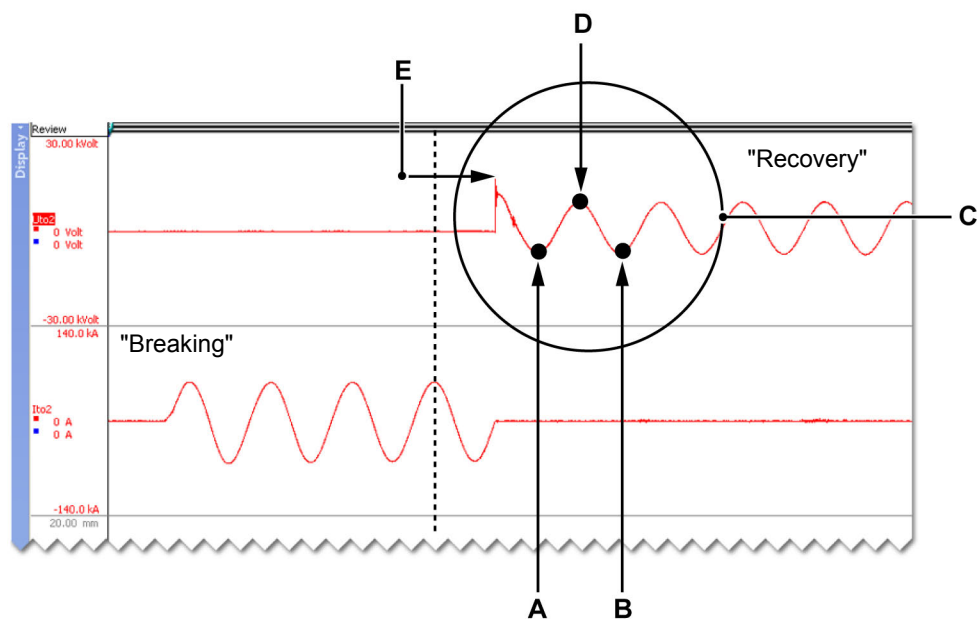
Figure 5.7: Display - Recovery voltage calculation
