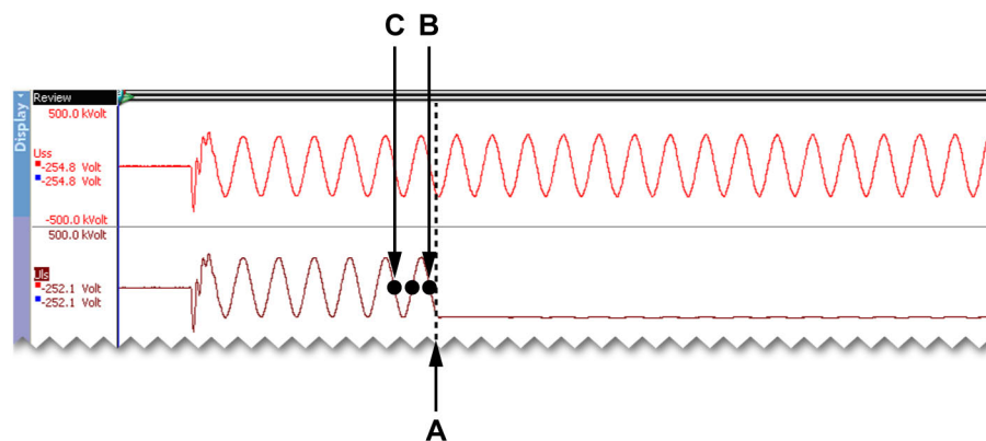
Figure 6.9: Display - Calculation on the voltage before contact separation (RMSTime)
