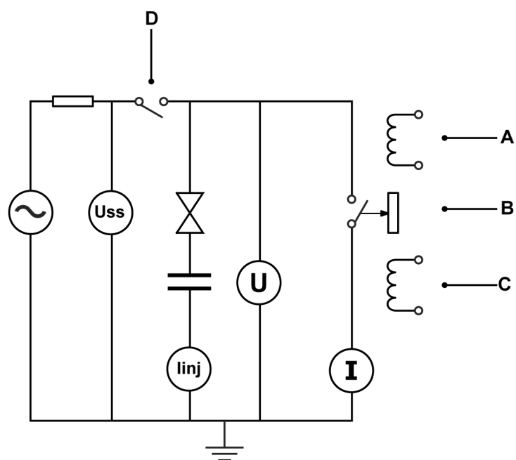
Figure 7.1: Diagram - Circuit breaker during a synthetic test
