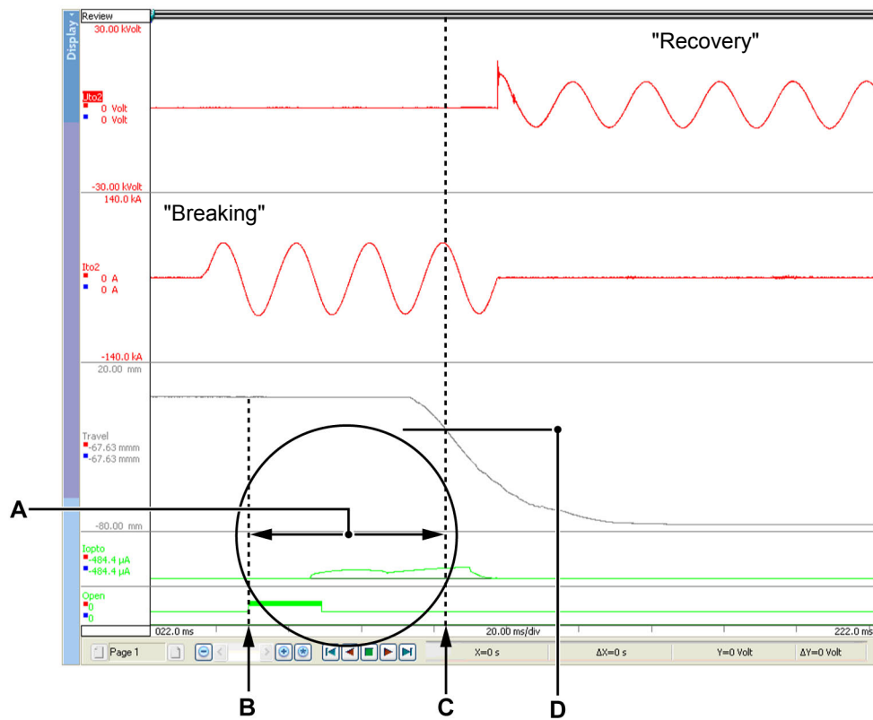
Figure 5.4: Display - Short circuit open event
