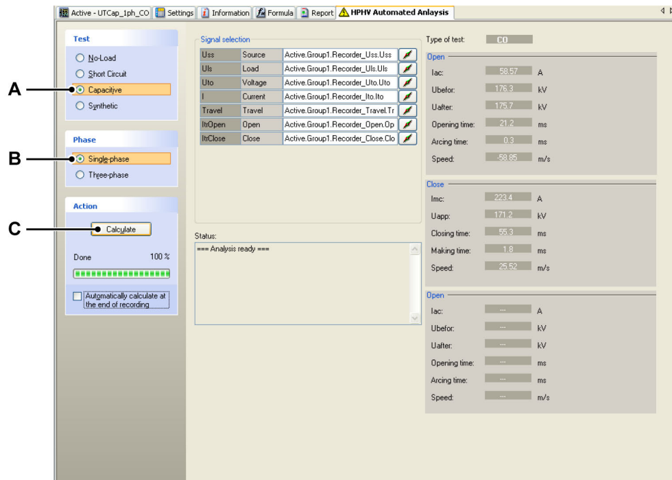
Figure 6.3: Perception HPHV window - Initial calculation process - Capacitive test
