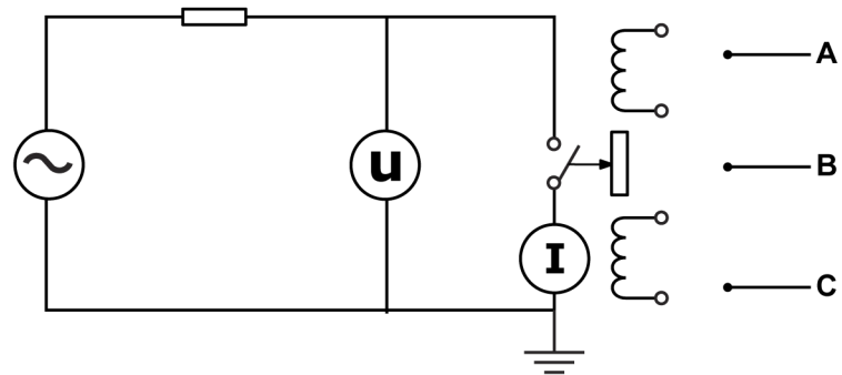
Figure 5.1: Diagram - Circuit breaker during a short circuit test
