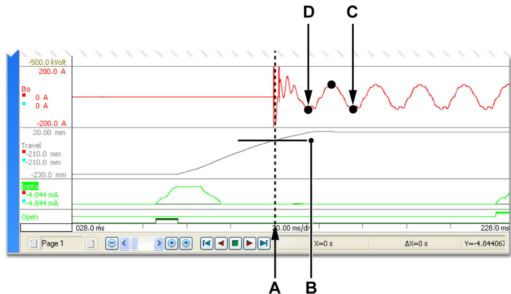
Figure 6.16: Display - Closing current calculations - RMS Time
