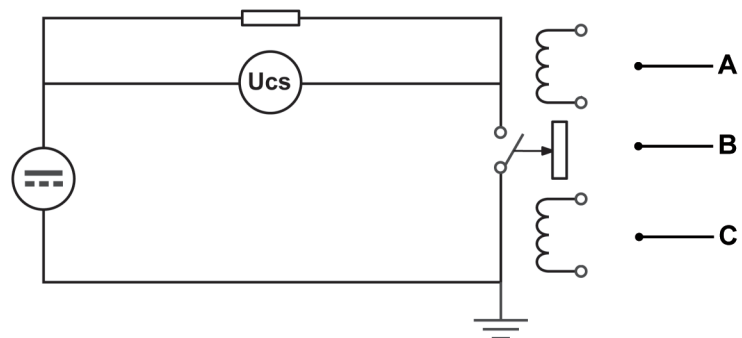
Figure 4.1: Diagram - Circuit breaker during a No-Load calculation
