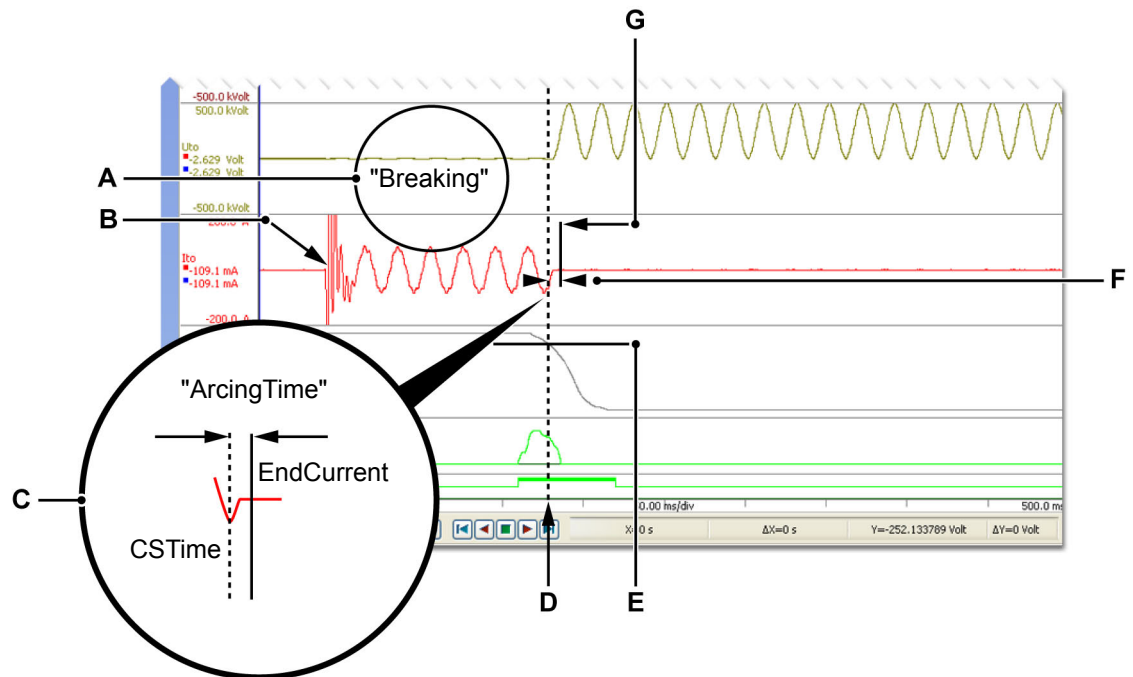
Figure 6.5: Display - Breaking current calculation process
