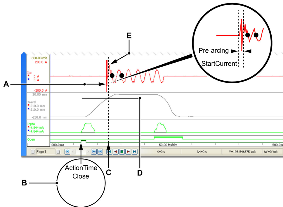
Figure 6.15: Display of a Close event - Capacitive test
