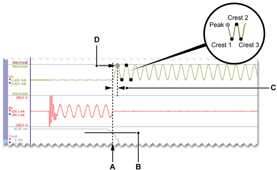
Figure 6.13: Display - Calculation on the voltage after contact separation (RMS Crests)
