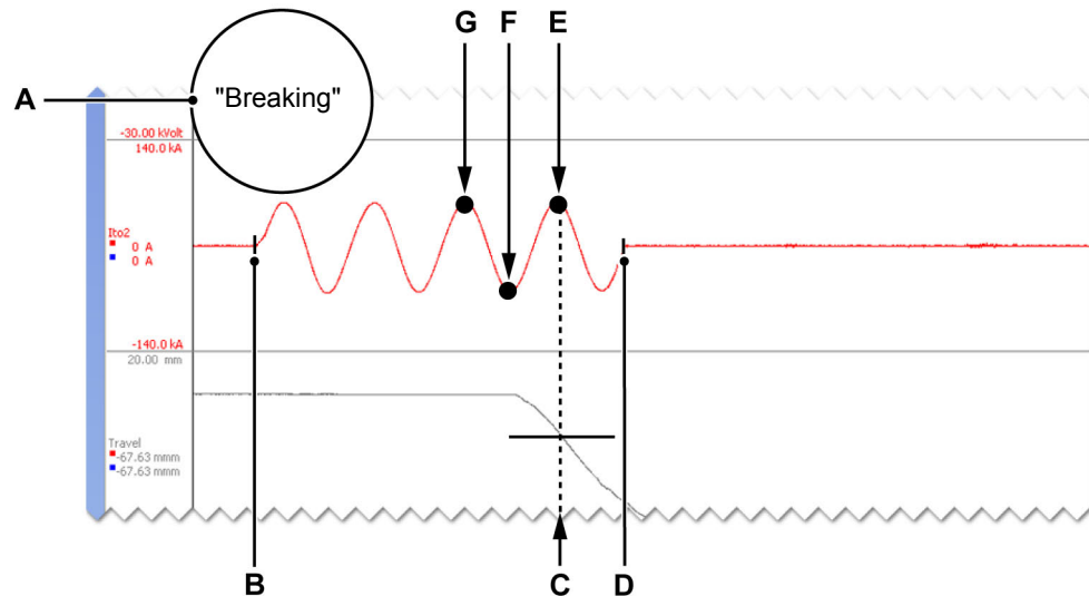
Figure 5.5: Display - Breaking current calculation process
