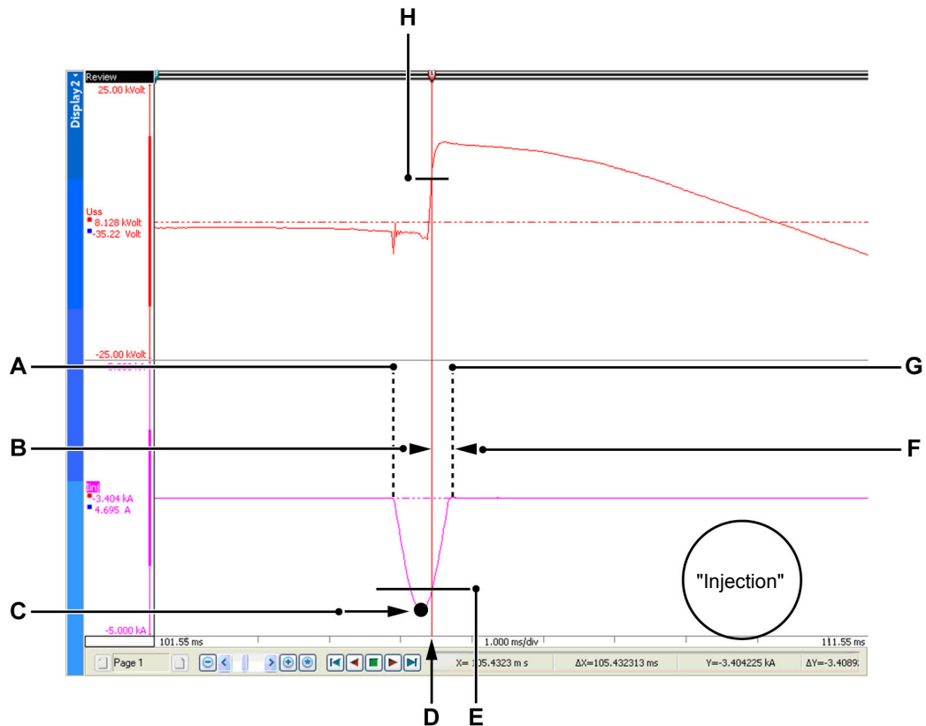
Figure 7.5: Display of an injection current - Synthetic test
