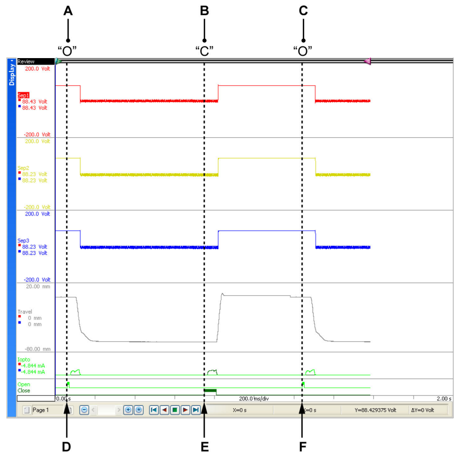
Figure 4.5: Display - Three-phase No-Load test
