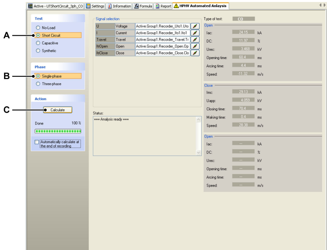
Figure 5.3: HPHV Automated Analysis sheet - Initial calculation process - Short circuit
