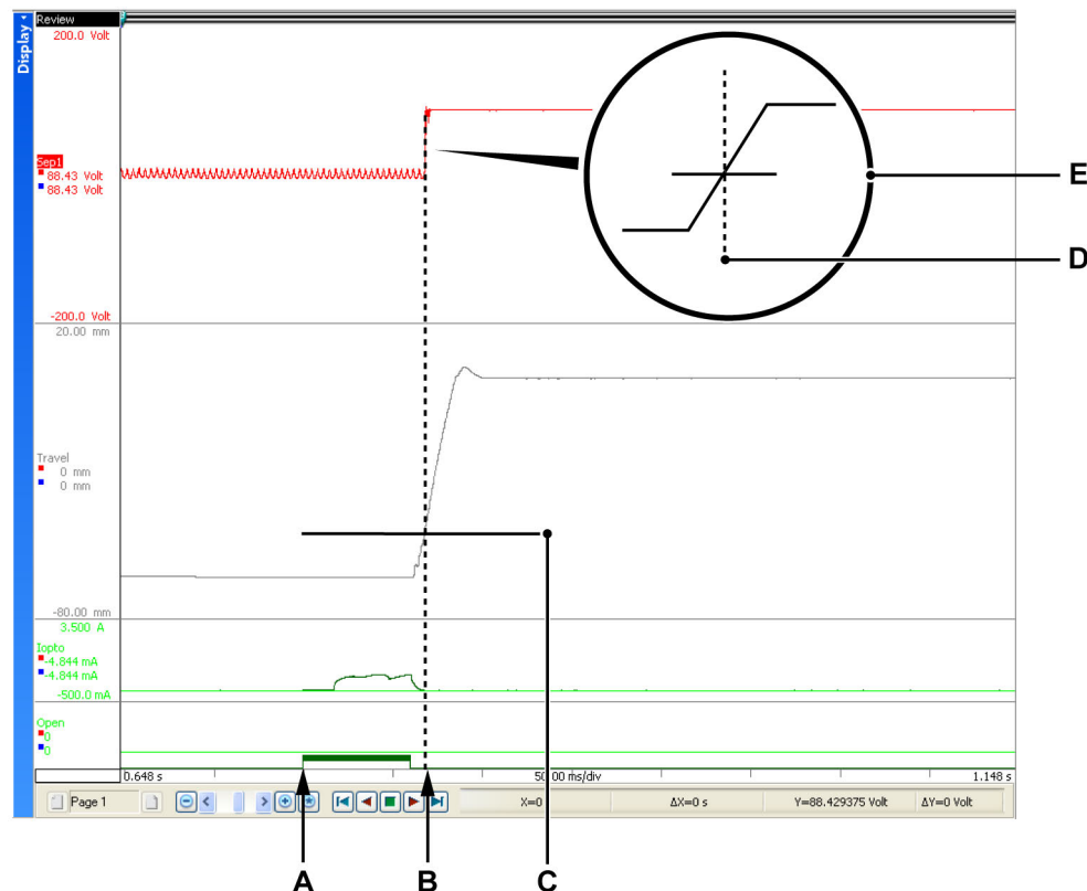
Figure 4.7: Display - Close event - Calculations on No-Load
