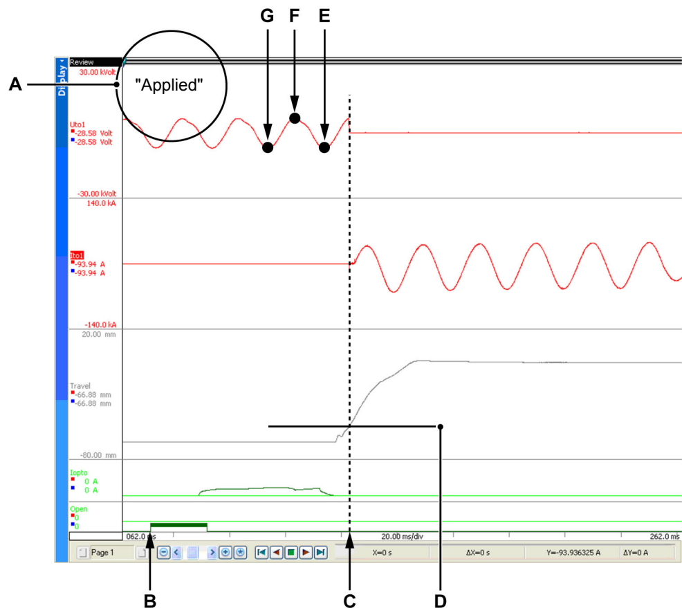
Figure 5.11: Display - Applied voltage calculation process
