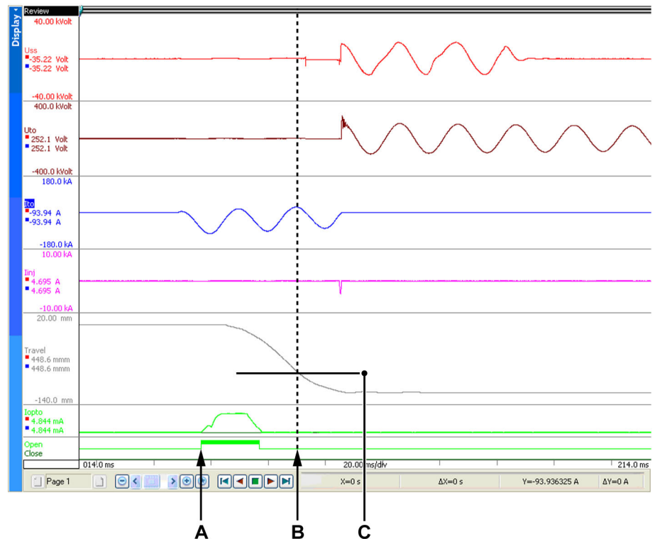
Figure 7.4: Display - Open event - Calculations for Synthetic test
