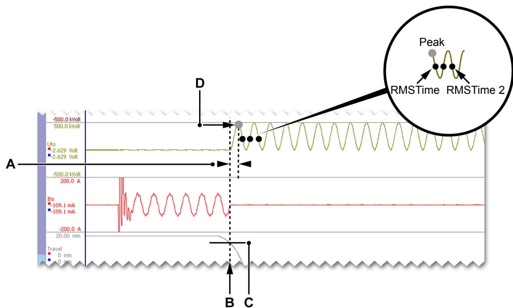
Figure 6.12: Display - Calculation on the voltage after contact separation (RMS Time)
