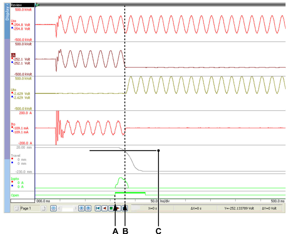
Figure 6.4: Display - Open event - Capacitive test
