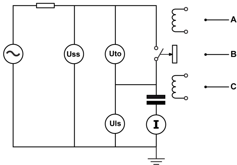
Figure 6.1: Diagram - Circuit breaker during a capacitive test
