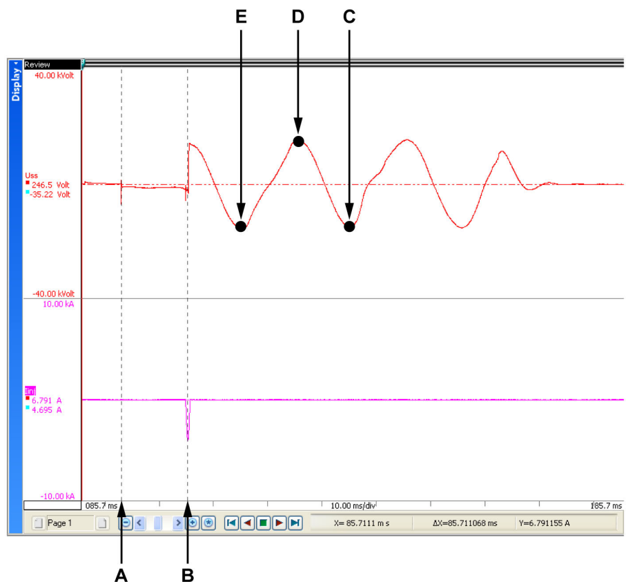
Figure 7.6: Display - Three-crest calculation on supply voltage
