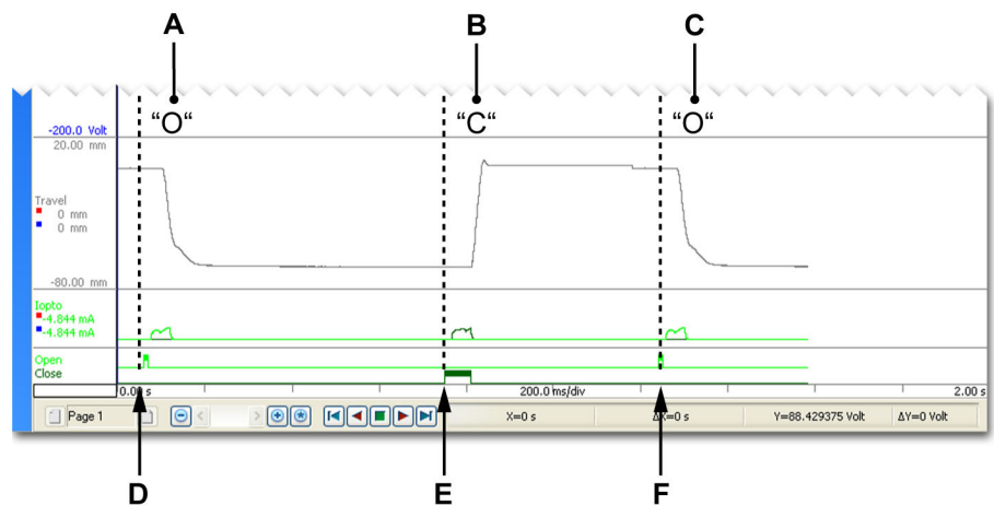
Figure 3.5: Display of the Travel Recorder Signal
