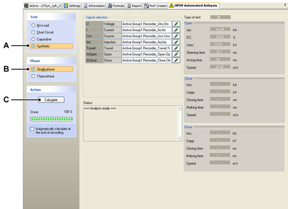
Figure 7.3: HPHV Automated Analysis Sheet - Initial calculation process - Synthetic test
