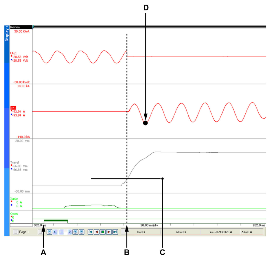
Figure 5.9: Display - Short circuit close event
