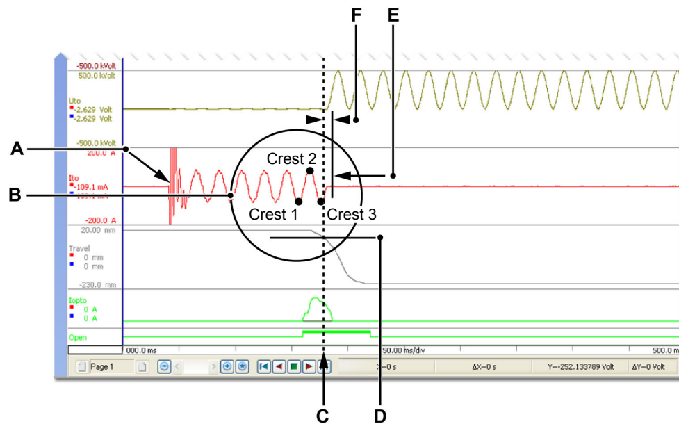
Figure 6.7: Display - Breaking current calculation process - Three-crest
