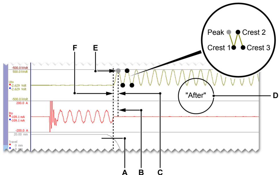
Figure 6.11: Display - Calculation on the voltage after contact separation
