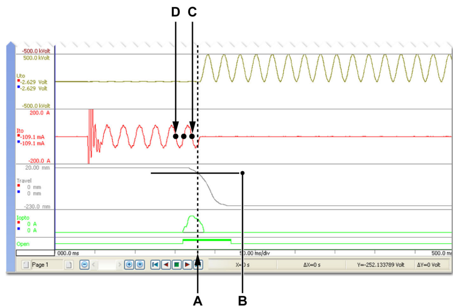
Figure 6.6: Display - Breaking current calculation process - RMS time
